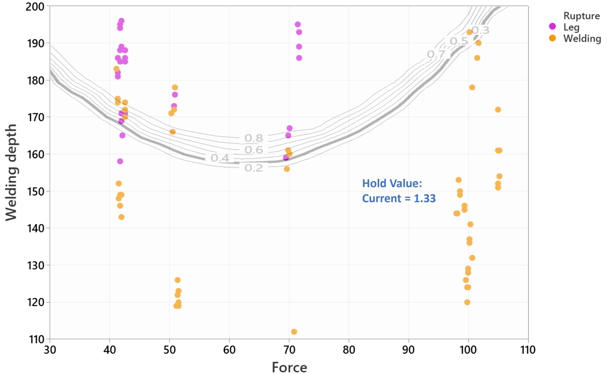
Scatterplot of Welding depth vs Force
