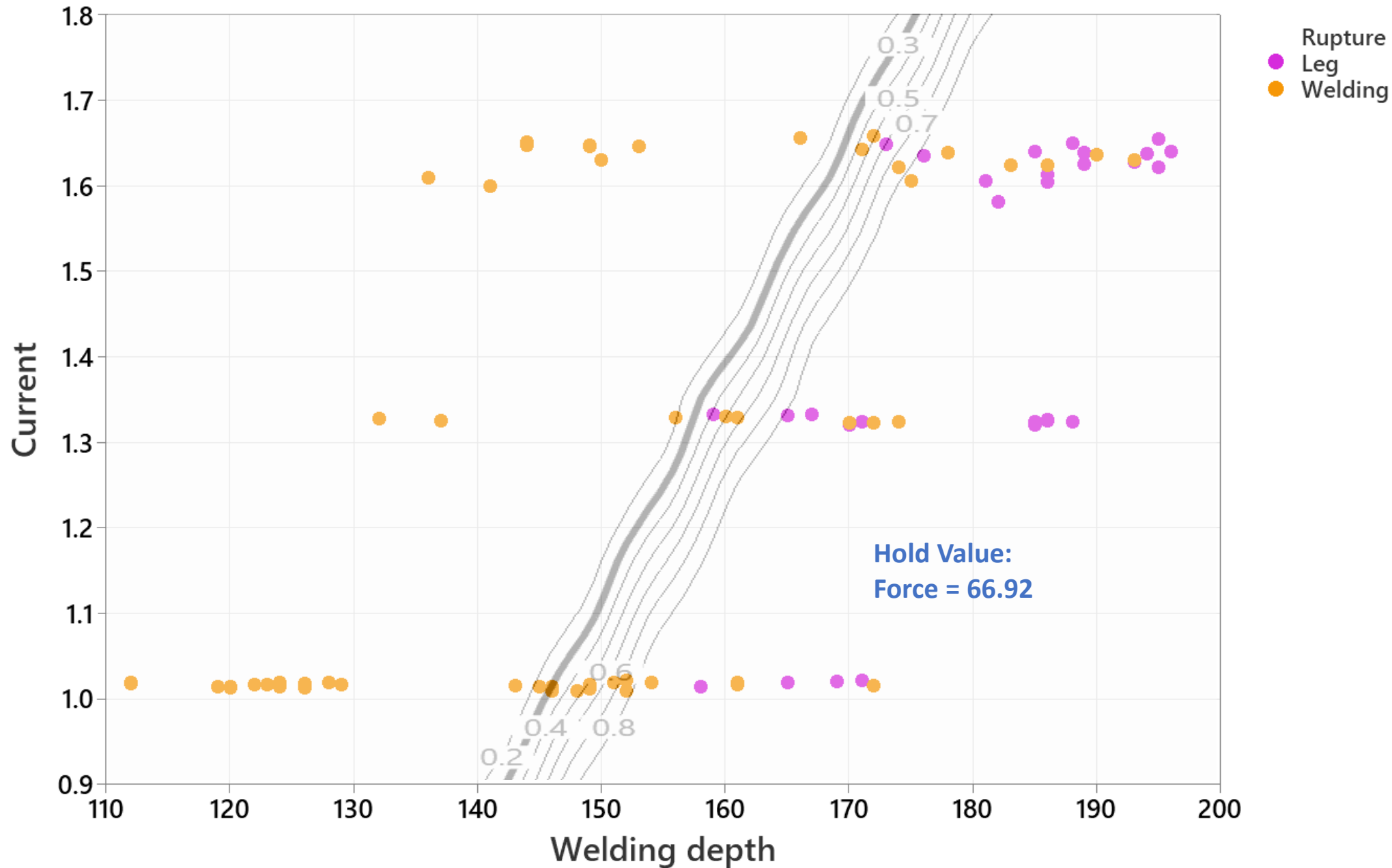
Scatterplot of Current vs Welding depth
